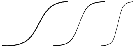
Figure 10.7 The shrinking S-curve.
